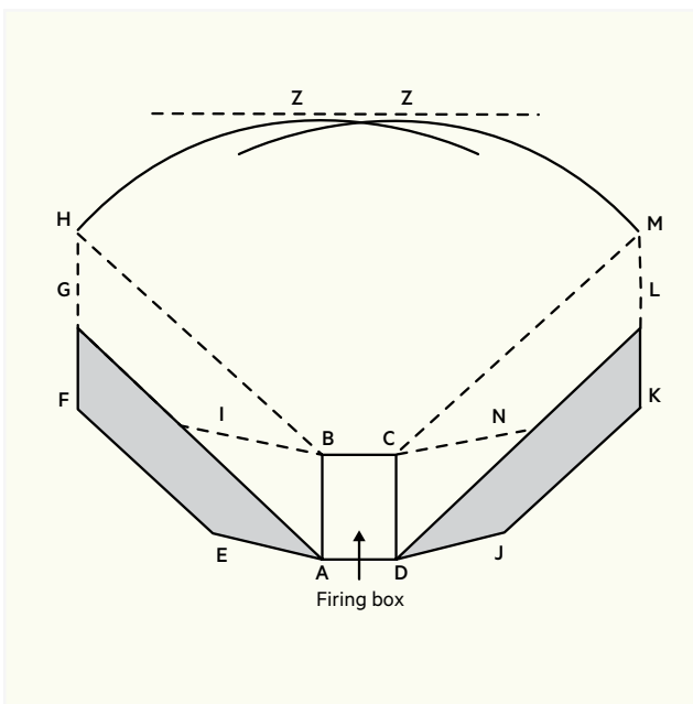
Figure 4.13 Example application of an ammunition danger area template from a firing box using parallel bearings with a maximum left and right of arc applied
