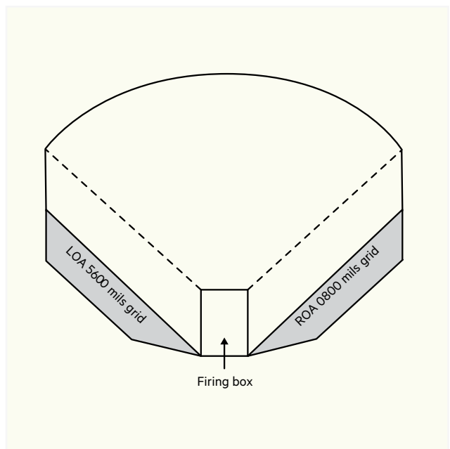
Figure 4.14 Example of a completed firing box using parallel bearings with maximum left and right of arcs
